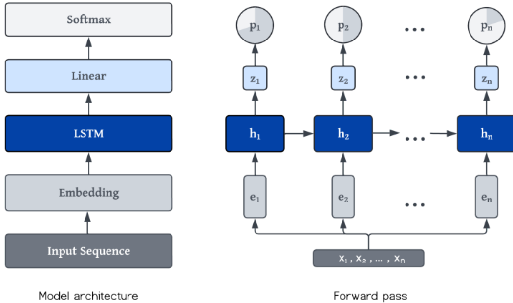
Figure 1. Model architecture (left) and forward pass (right). The left panel outlines the structural components of the model, while the right illustrates the flow of data and transformations applied at each stage.
