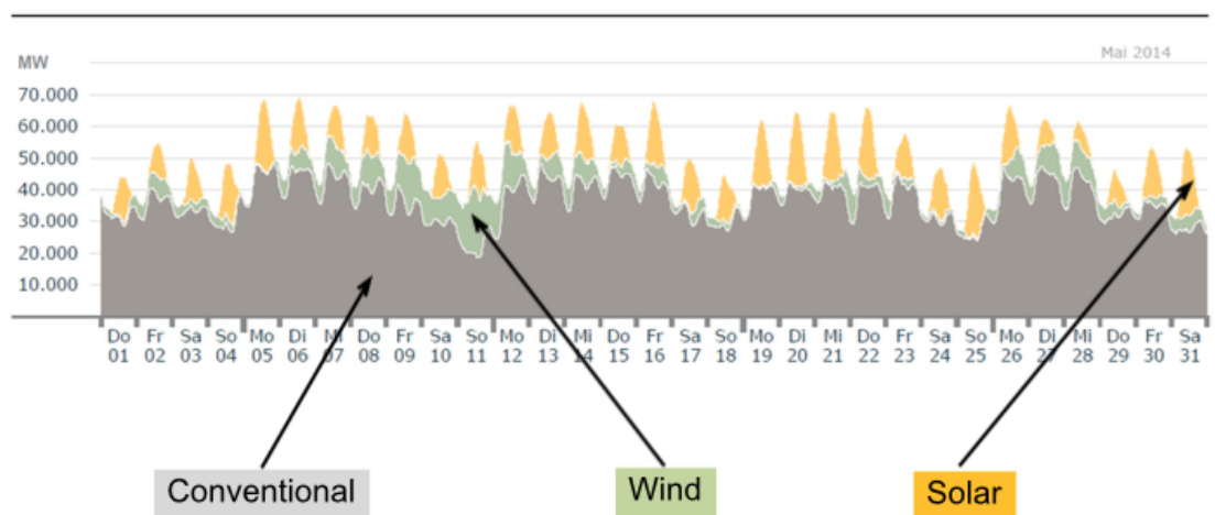
Fluctuations in Power Production, Germany (Mai 2014)
