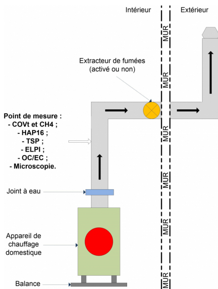
Figure 4. Description de la plate-forme expérimentale. Description of the experimental platform.
